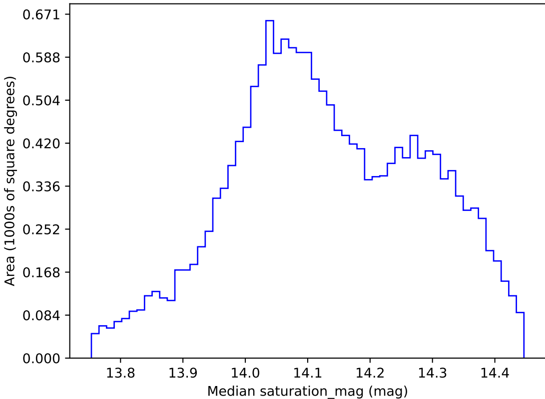
too_ignore_5_1v3.4_10yrs WFD z band: Median saturation_mag
