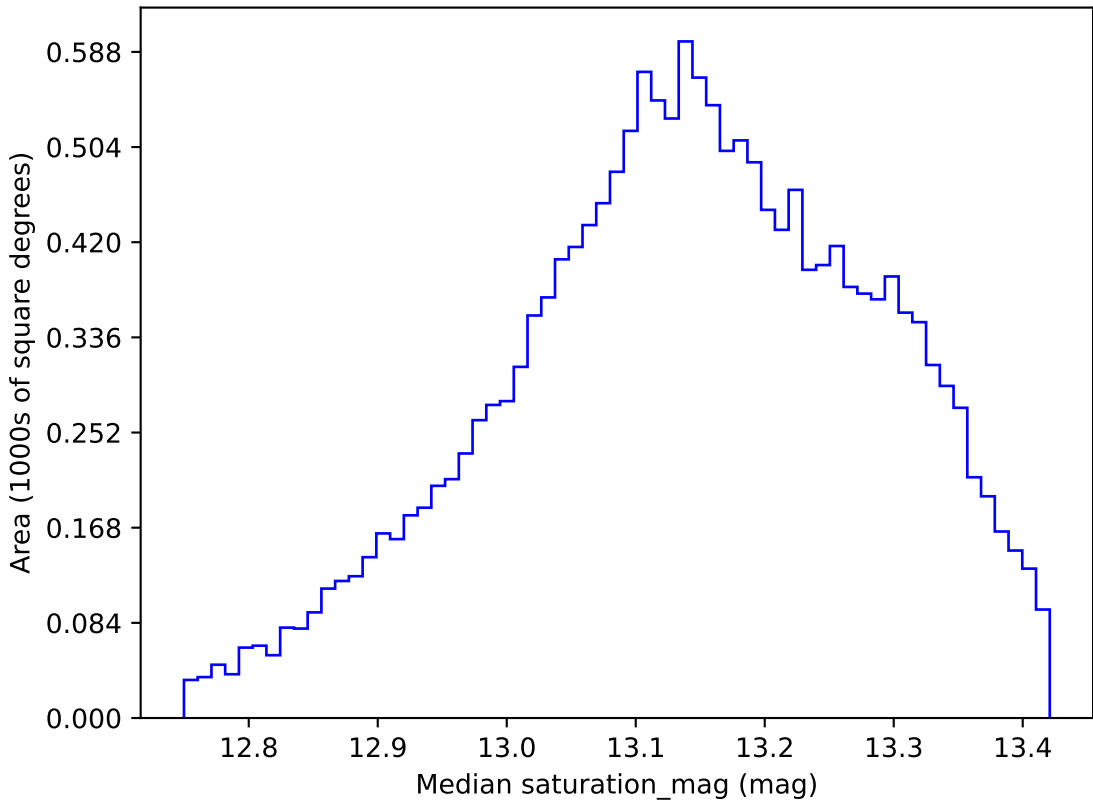
too_ignore_5_1v3.4_10yrs WFD y band: Median saturation_mag
