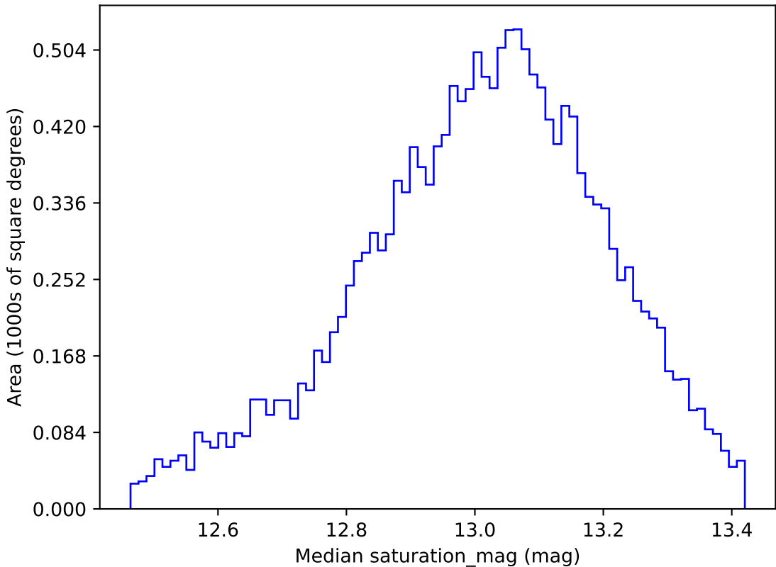
too_ignore_5_1v3.4_10yrs WFD u band: Median saturation_mag
