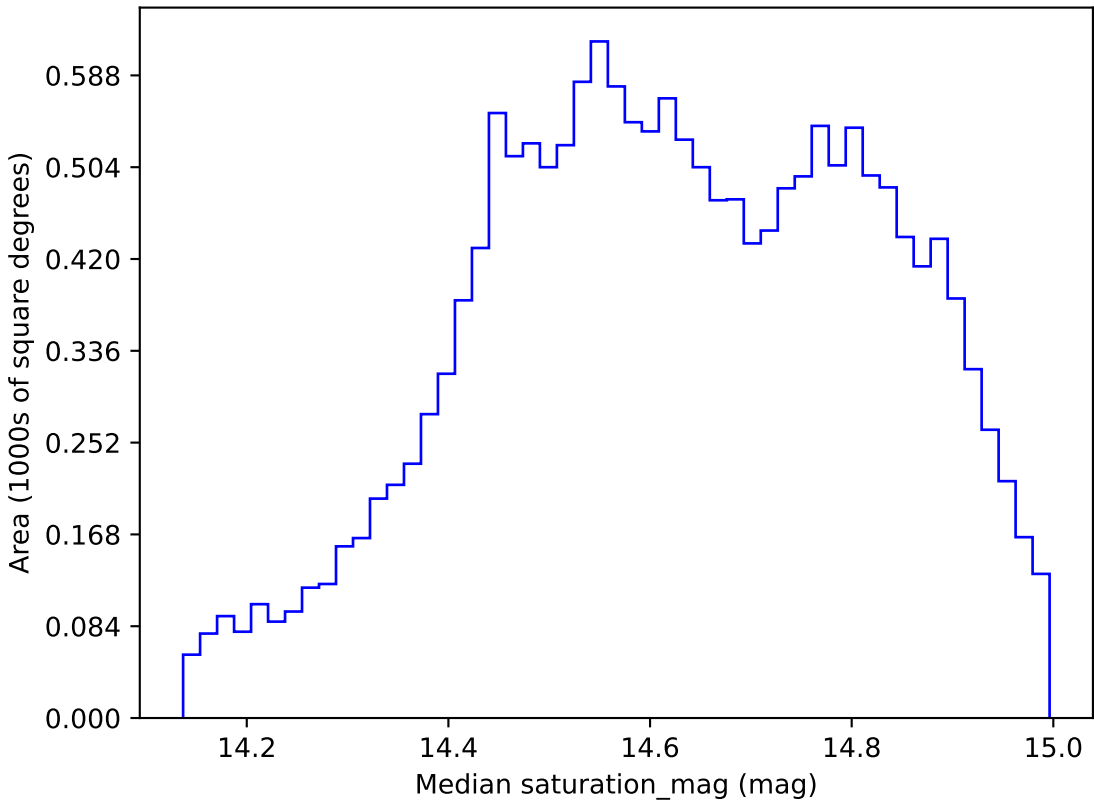
too_ignore_5_1v3.4_10yrs WFD r band: Median saturation_mag
