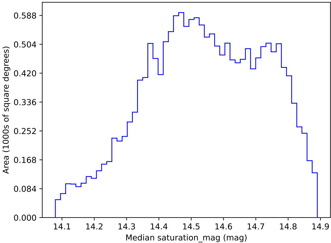
too_ignore_5_1v3.4_10yrs WFD i band: Median saturation_mag
