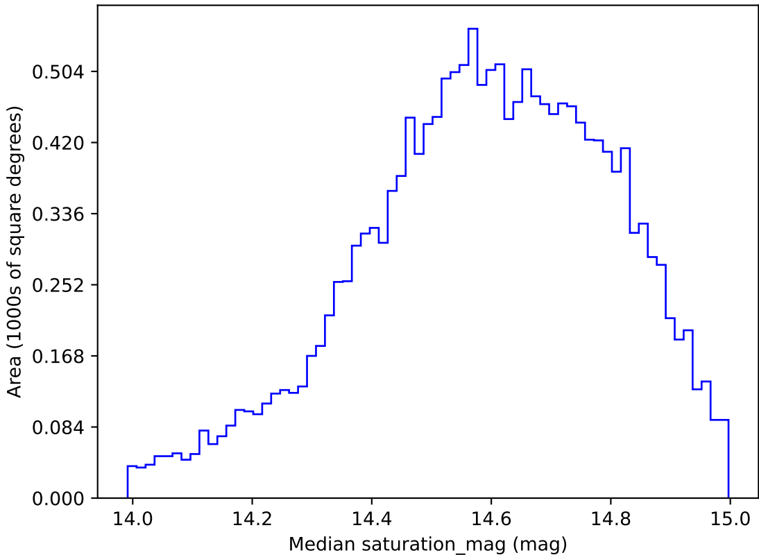
too_ignore_5_1v3.4_10yrs WFD g band: Median saturation_mag
