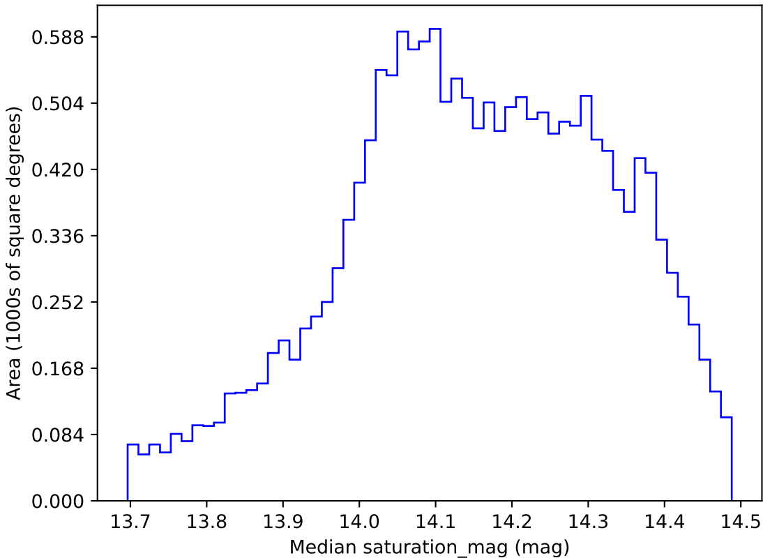
too_ignore_5_1v3.4_10yrs WFD all bands: Median saturation_mag
