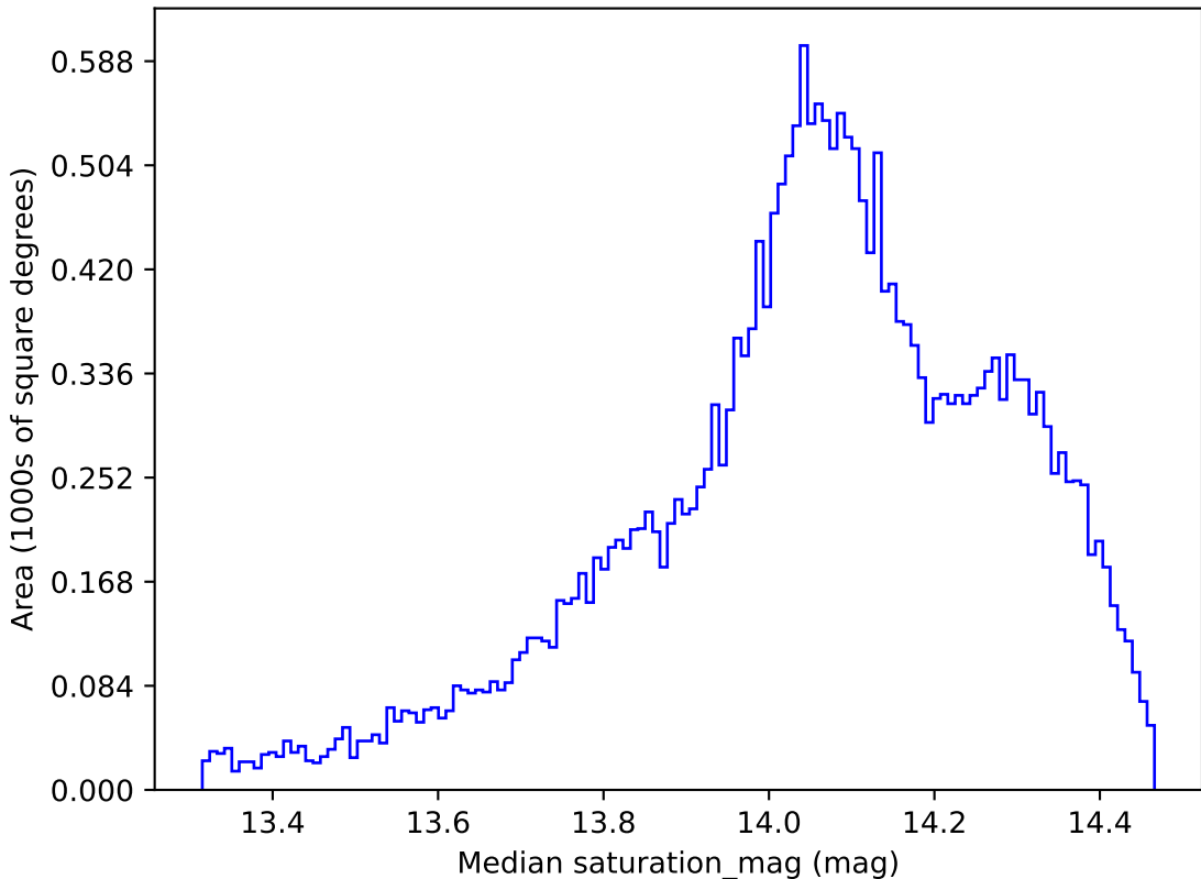
too_ignore_5_1v3.4_10yrs All sky z band: Median saturation_mag
