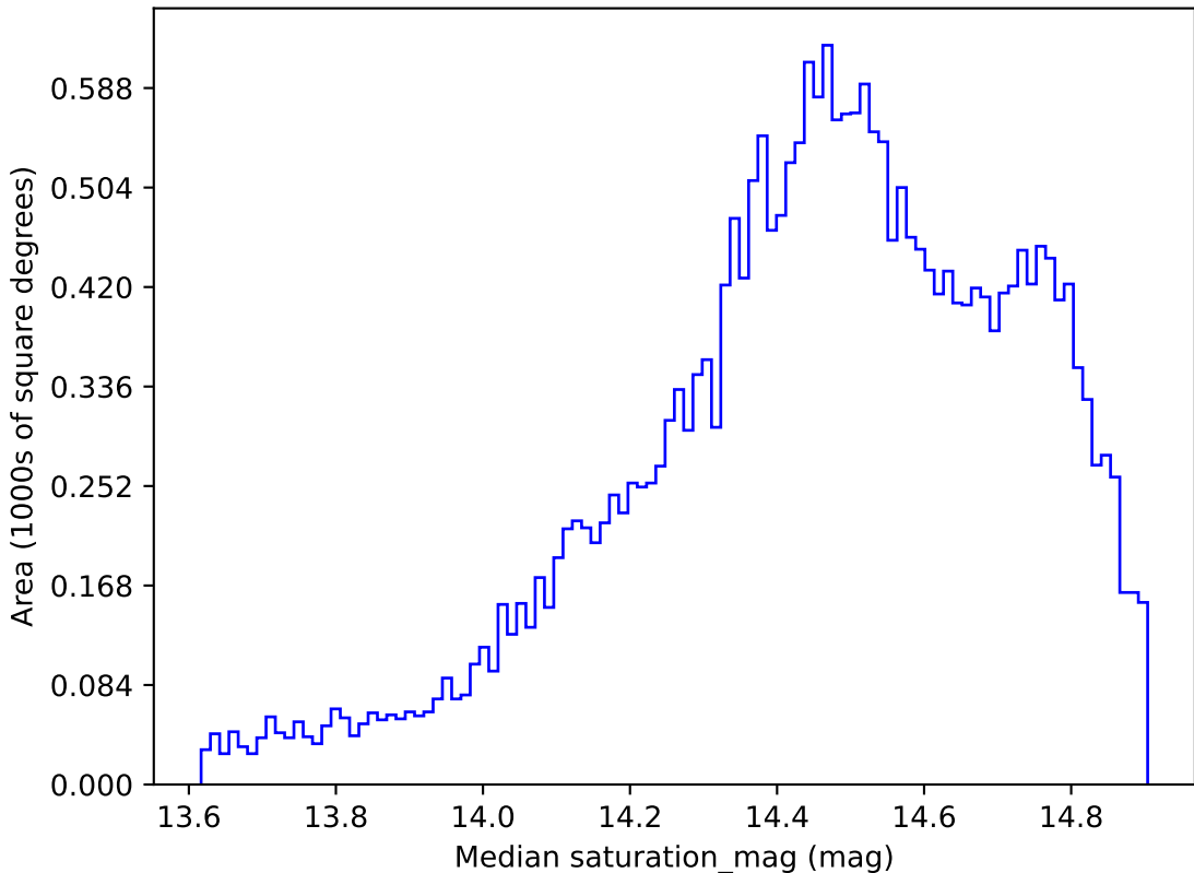
too_ignore_5_1v3.4_10yrs All sky i band: Median saturation_mag
