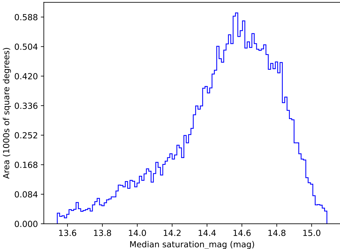
too_ignore_5_1v3.4_10yrs All sky g band: Median saturation_mag
