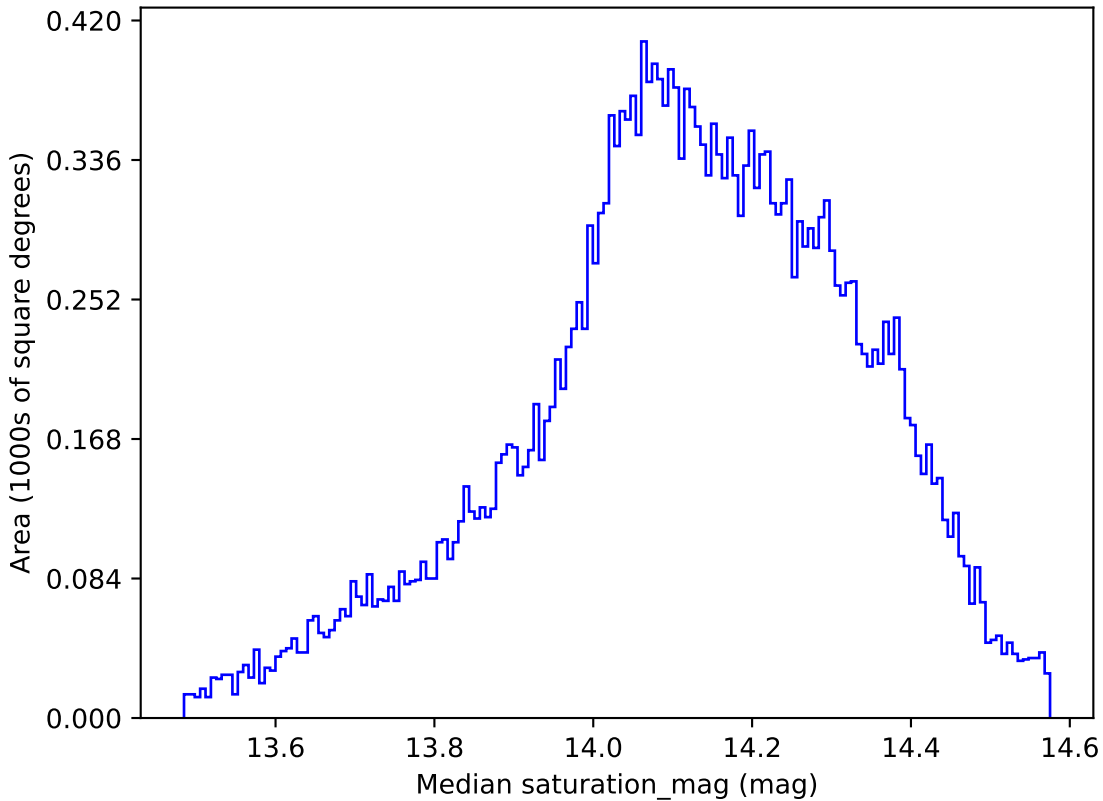
too_ignore_5_1v3.4_10yrs All sky all bands: Median saturation_mag
