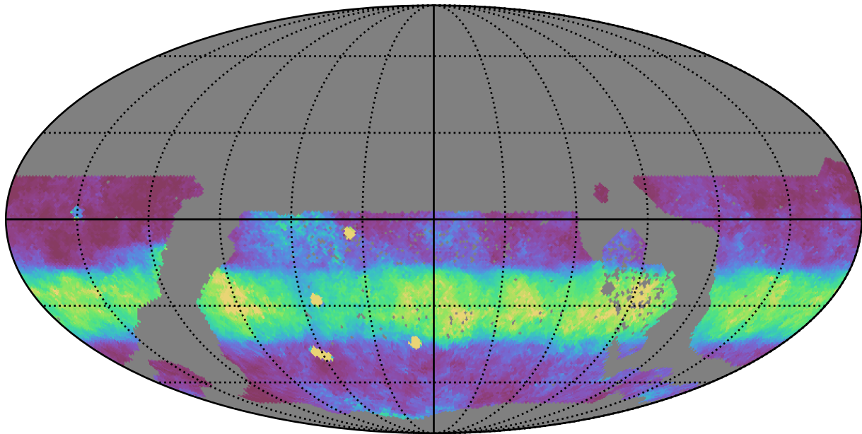
too_ignore_5_1v3.4_10yrs WFD z band: Median normairmass
