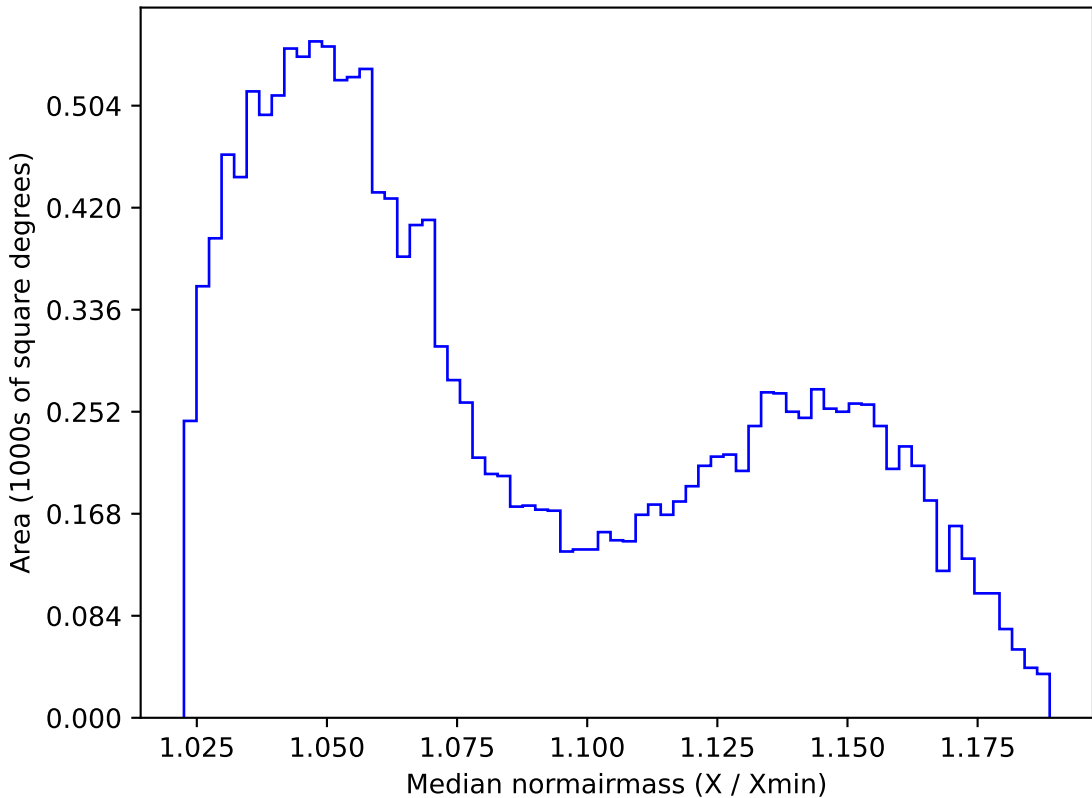
too_ignore_5_1v3.4_10yrs WFD z band: Median normairmass
