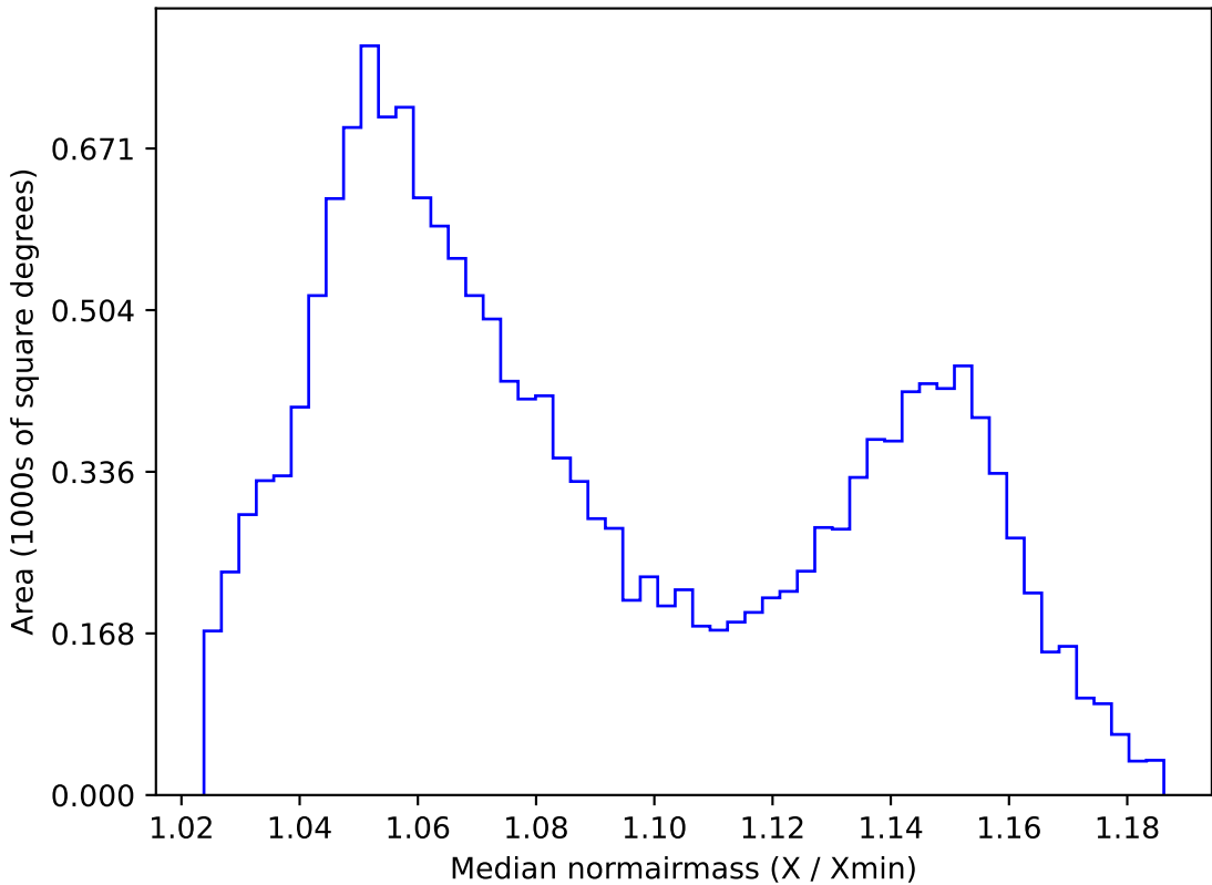
too_ignore_5_1v3.4_10yrs WFD y band: Median normairmass
