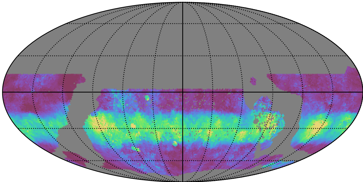
too_ignore_5_1v3.4_10yrs WFD u band: Median normairmass
