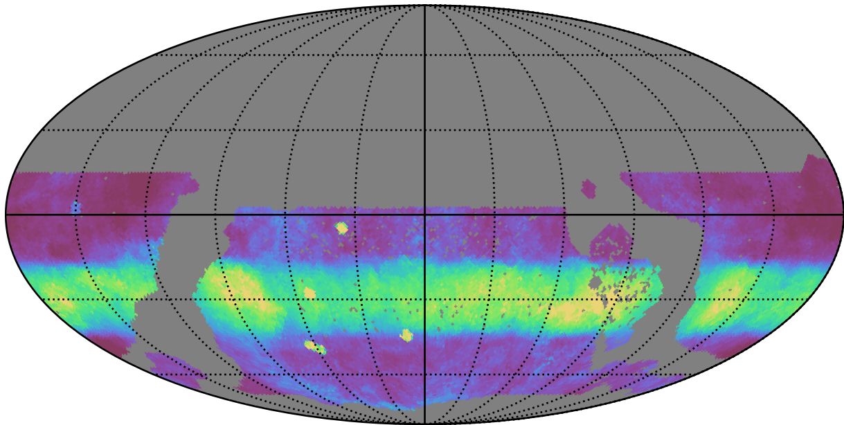
too_ignore_5_1v3.4_10yrs WFD r band: Median normairmass
