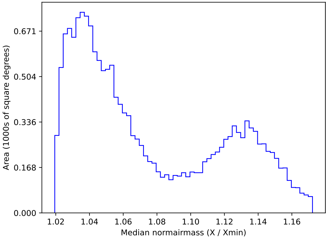
too_ignore_5_1v3.4_10yrs WFD i band: Median normairmass
