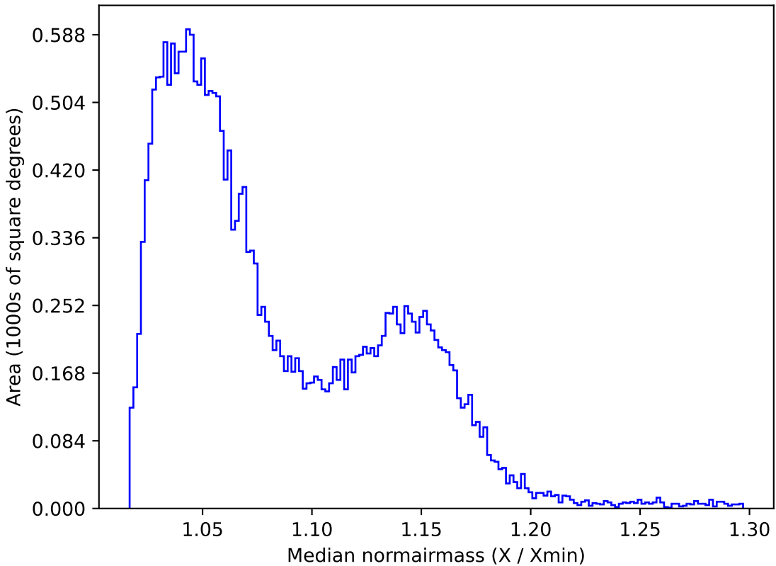
too_ignore_5_1v3.4_10yrs All sky z band: Median normairmass
