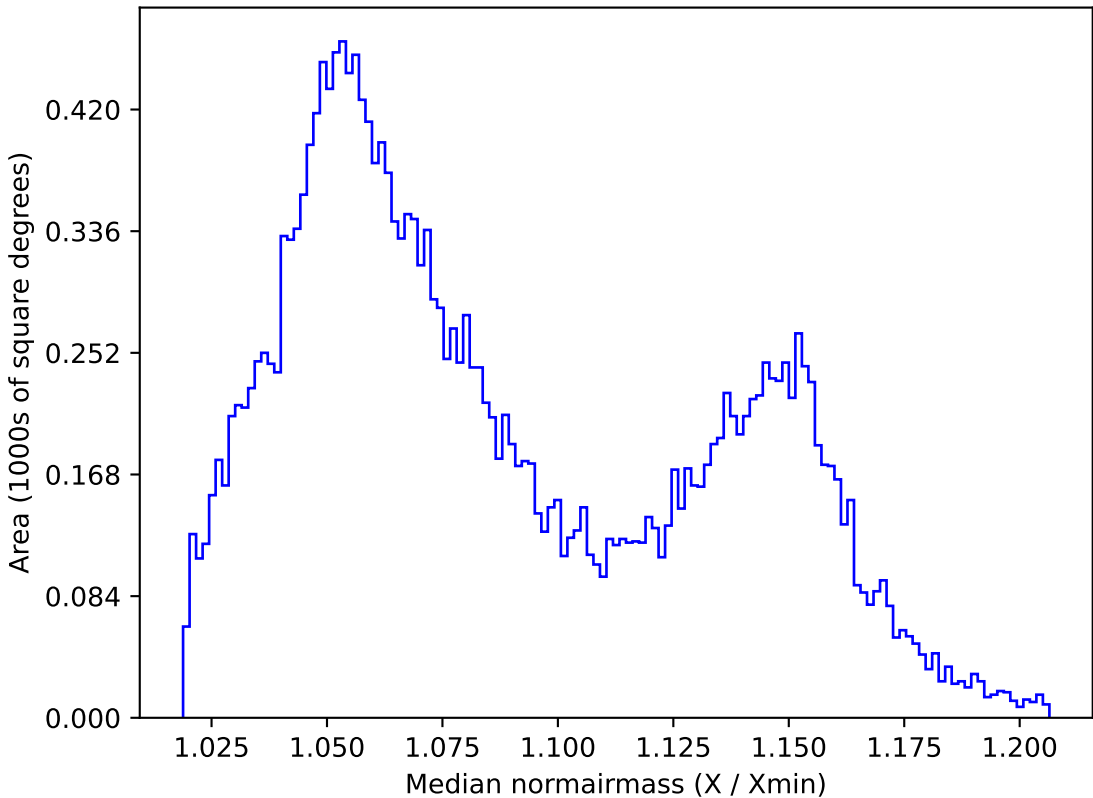
too_ignore_5_1v3.4_10yrs All sky y band: Median normairmass
