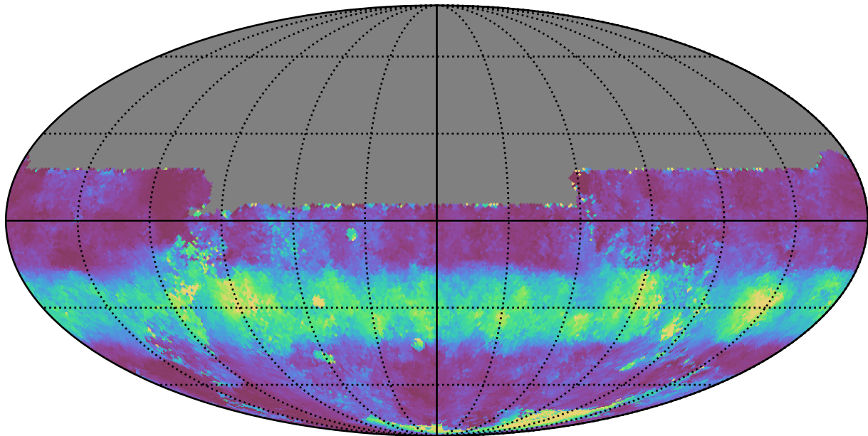
too_ignore_5_1v3.4_10yrs All sky u band: Median normairmass
