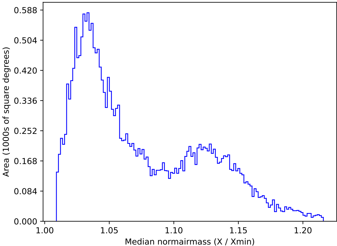
too_ignore_5_1v3.4_10yrs All sky u band: Median normairmass
