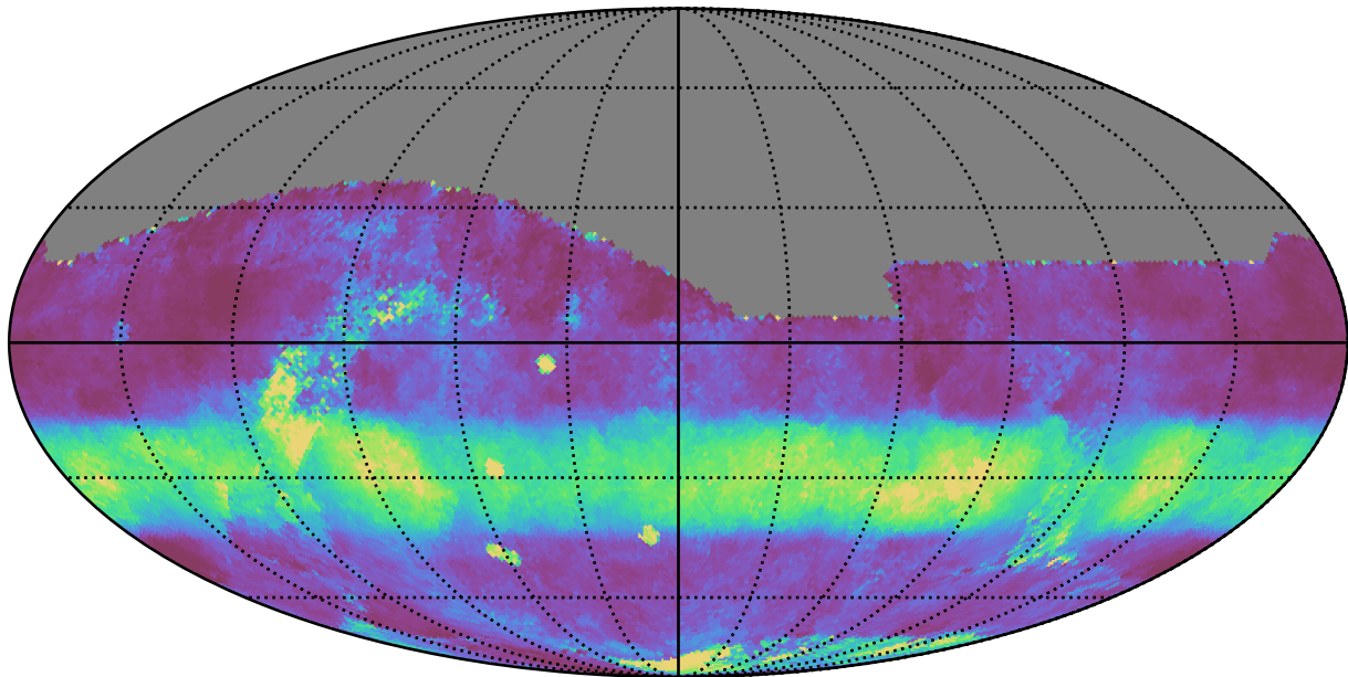
too_ignore_5_1v3.4_10yrs All sky r band: Median normairmass
