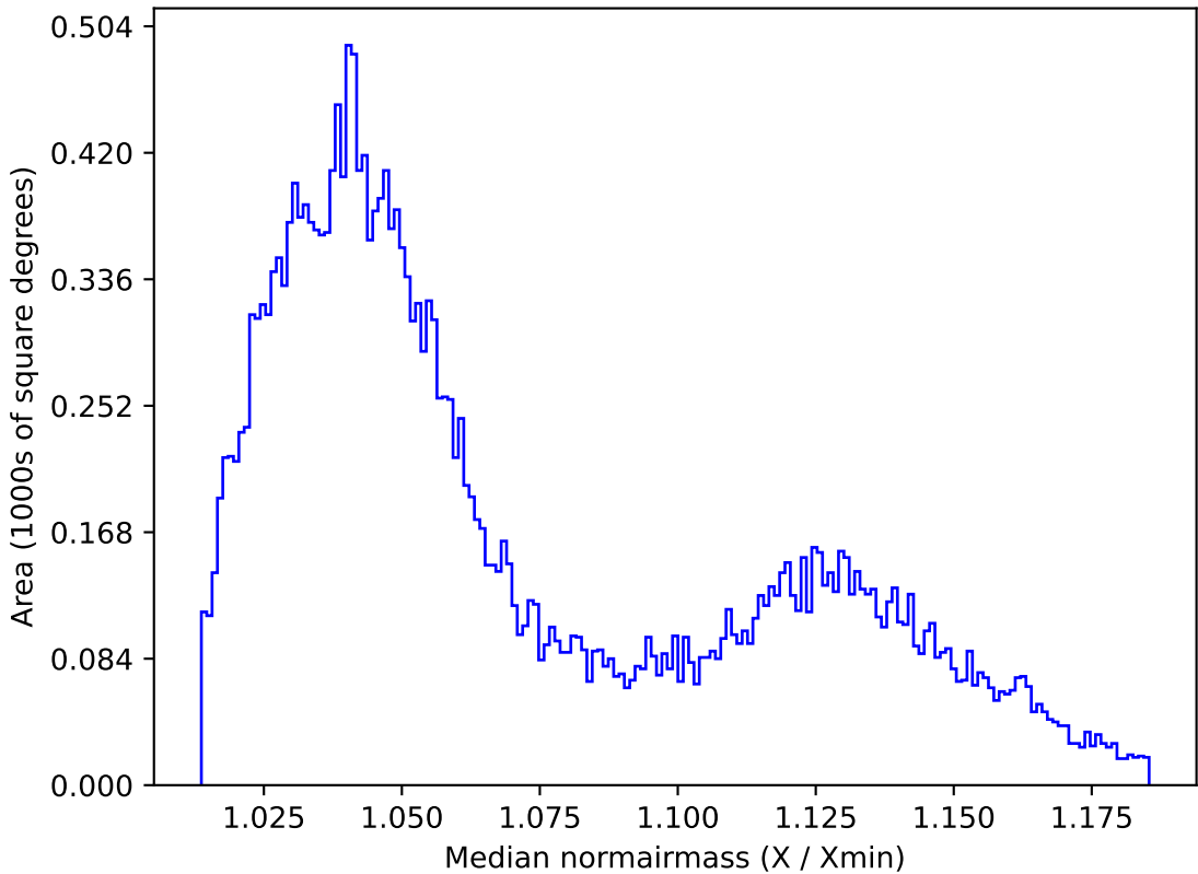
too_ignore_5_1v3.4_10yrs All sky r band: Median normairmass
