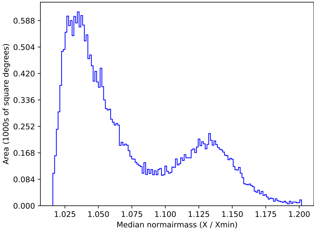
too_ignore_5_1v3.4_10yrs All sky i band: Median normairmass
