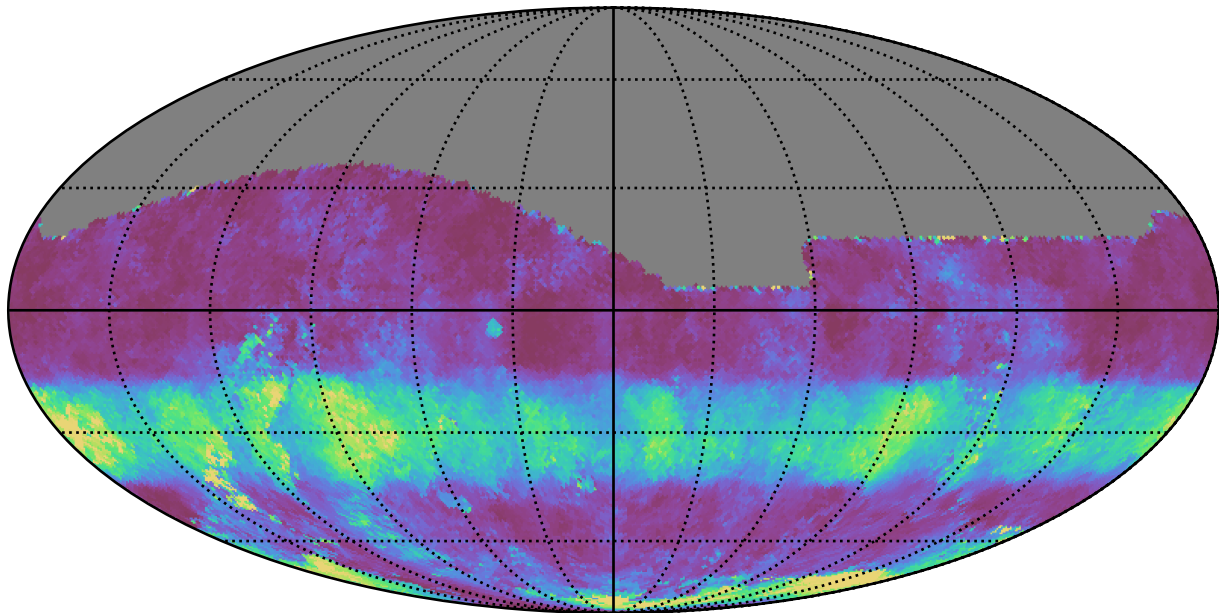
too_ignore_5_1v3.4_10yrs All sky g band: Median normairmass
