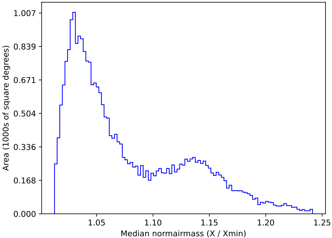
too_ignore_5_1v3.4_10yrs All sky g band: Median normairmass
