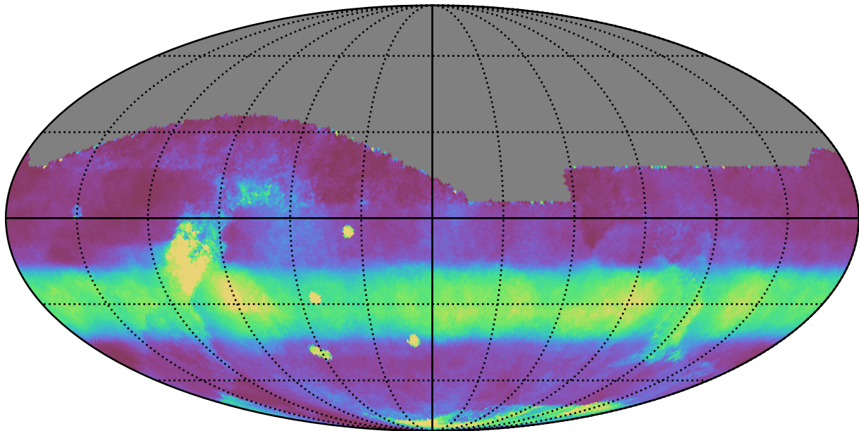
too_ignore_5_1v3.4_10yrs All sky all bands: Median normairmass
