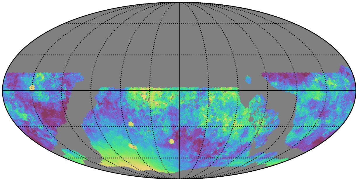
too_ignore_5_1v3.4_10yrs WFD z band: Median moonDistance
