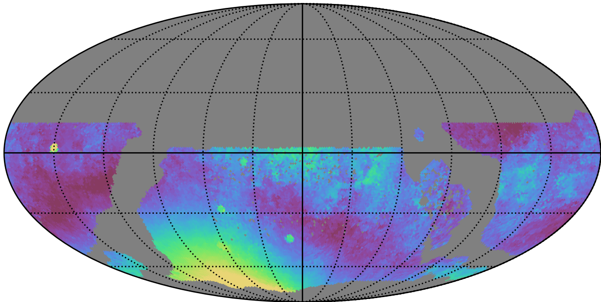
too_ignore_5_1v3.4_10yrs WFD y band: Median moonDistance
