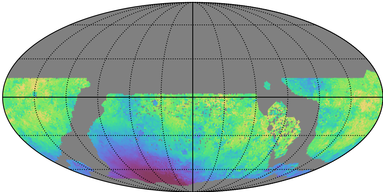
too_ignore_5_1v3.4_10yrs WFD u band: Median moonDistance
