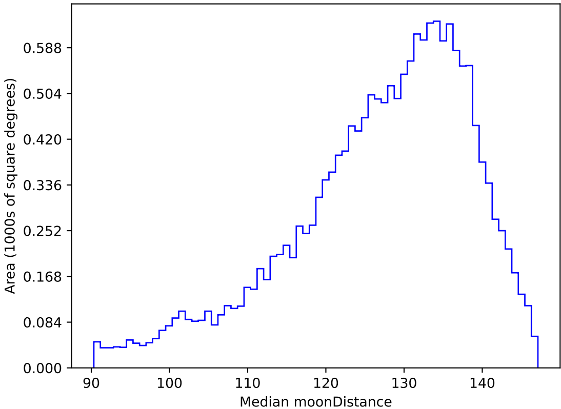
too_ignore_5_1v3.4_10yrs WFD u band: Median moonDistance
