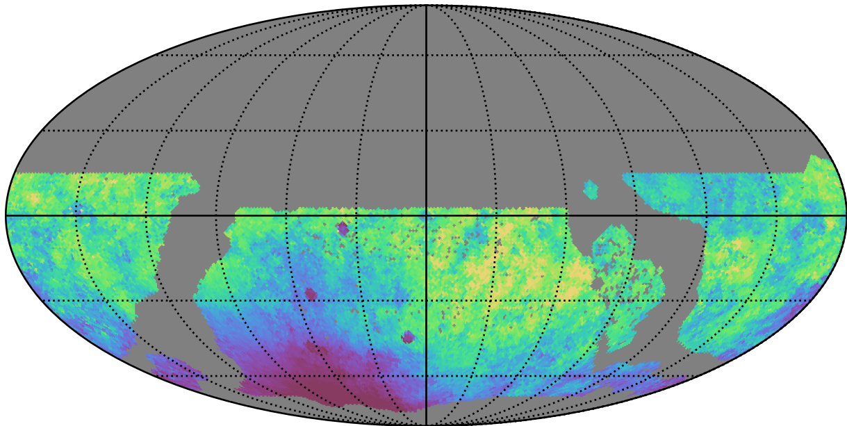
too_ignore_5_1v3.4_10yrs WFD r band: Median moonDistance
