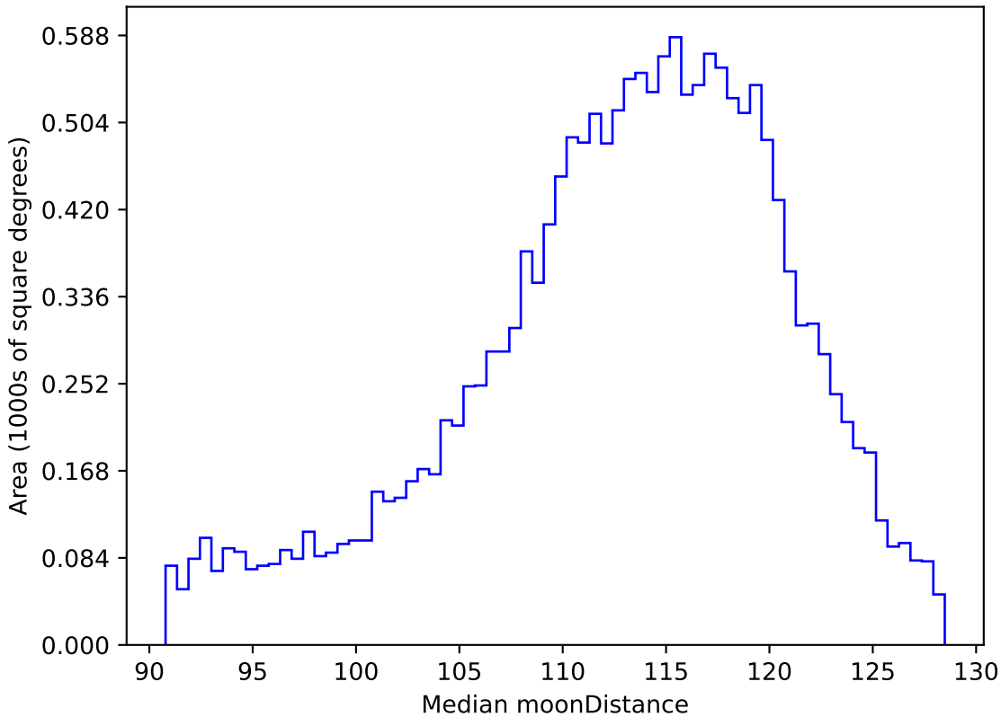
too_ignore_5_1v3.4_10yrs WFD r band: Median moonDistance
