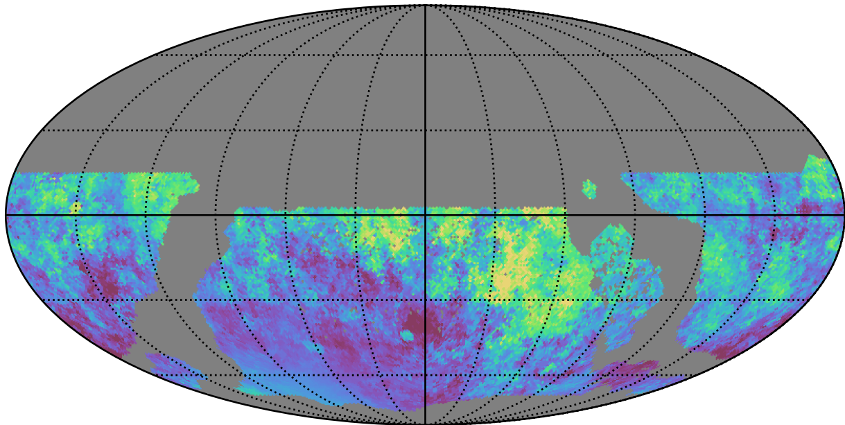
too_ignore_5_1v3.4_10yrs WFD i band: Median moonDistance
