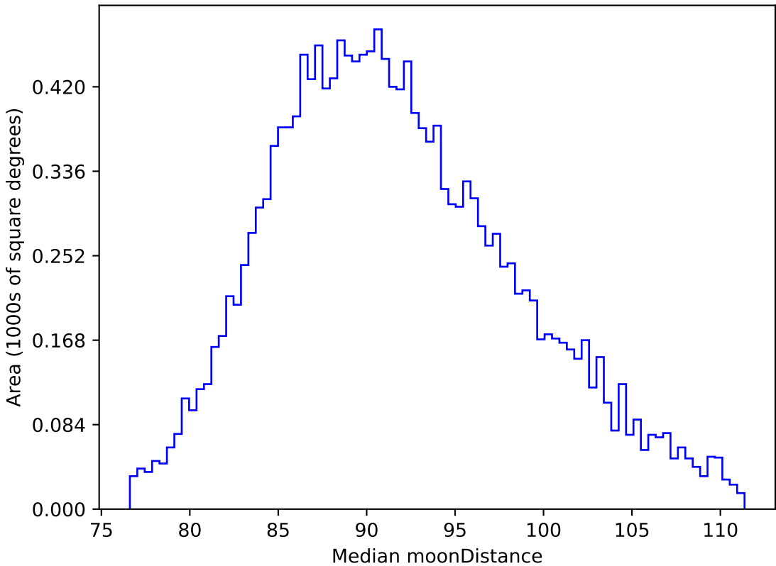
too_ignore_5_1v3.4_10yrs WFD i band: Median moonDistance
