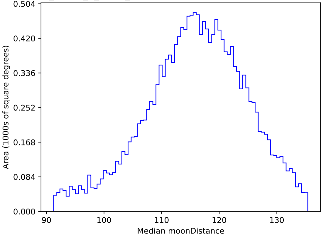
too_ignore_5_1v3.4_10yrs WFD g band: Median moonDistance
