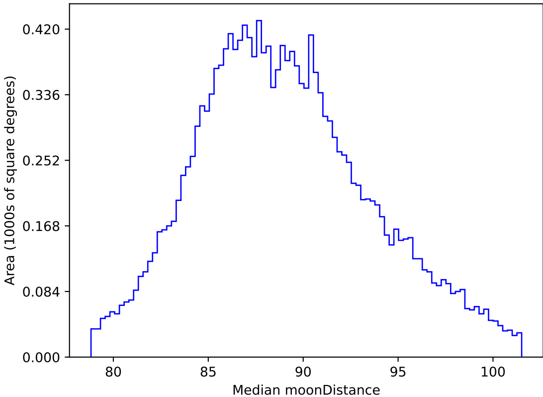
too_ignore_5_1v3.4_10yrs WFD all bands: Median moonDistance
