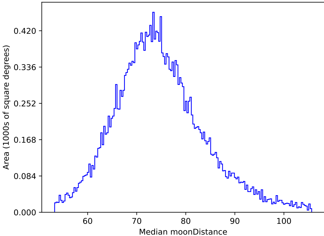
too_ignore_5_1v3.4_10yrs All sky z band: Median moonDistance
