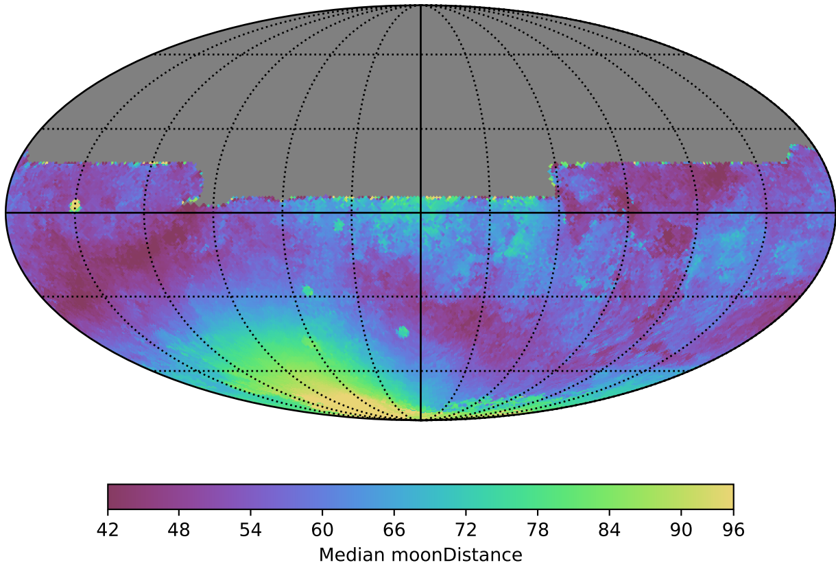
too_ignore_5_1v3.4_10yrs All sky y band: Median moonDistance
