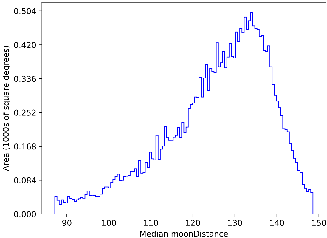
too_ignore_5_1v3.4_10yrs All sky u band: Median moonDistance
