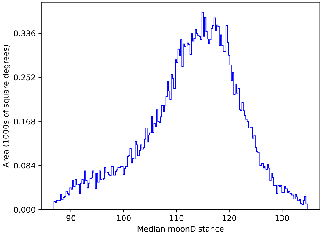
too_ignore_5_1v3.4_10yrs All sky r band: Median moonDistance
