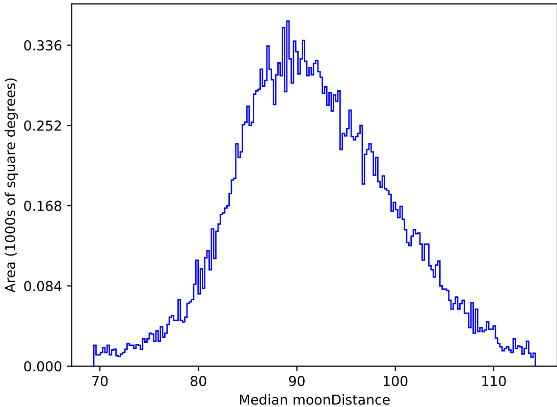
too_ignore_5_1v3.4_10yrs All sky i band: Median moonDistance
