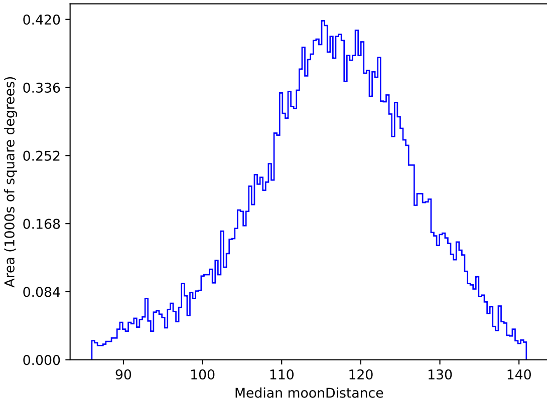
too_ignore_5_1v3.4_10yrs All sky g band: Median moonDistance
