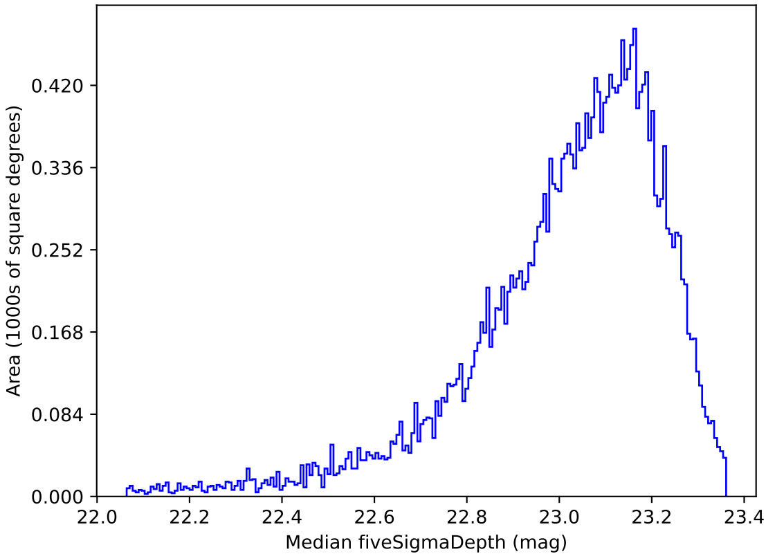
too_ignore_5_1v3.4_10yrs Yr 1 z band: Median fiveSigmaDepth
