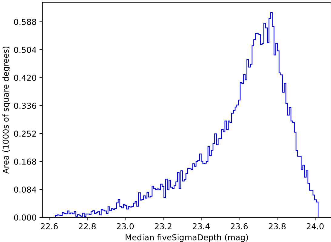
too_ignore_5_1v3.4_10yrs Yr 1 i band: Median fiveSigmaDepth
