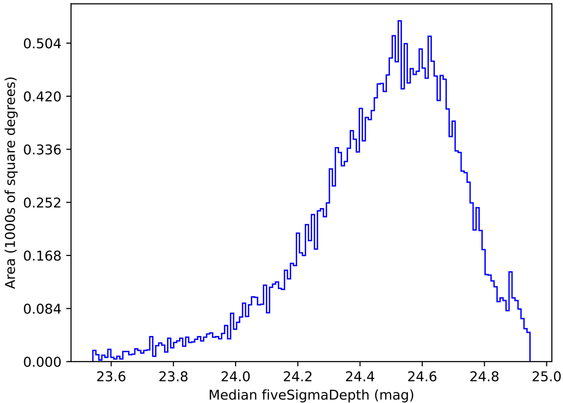
too_ignore_5_1v3.4_10yrs Yr 1 g band: Median fiveSigmaDepth
