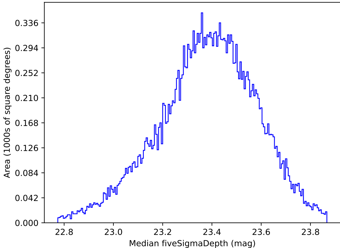
too_ignore_5_1v3.4_10yrs Yr 1 all bands: Median fiveSigmaDepth
