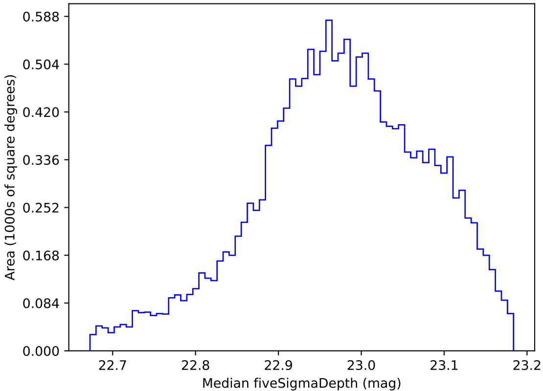
too_ignore_5_1v3.4_10yrs WFD z band: Median fiveSigmaDepth
