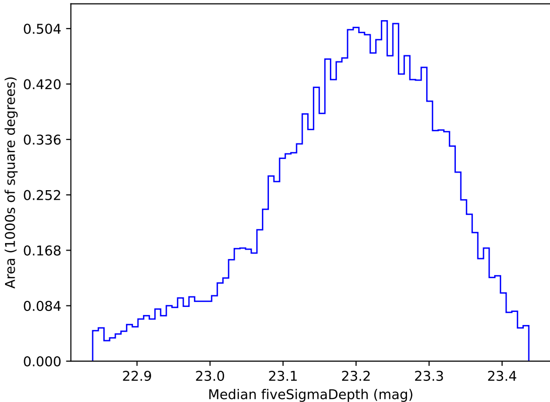
too_ignore_5_1v3.4_10yrs WFD u band: Median fiveSigmaDepth
