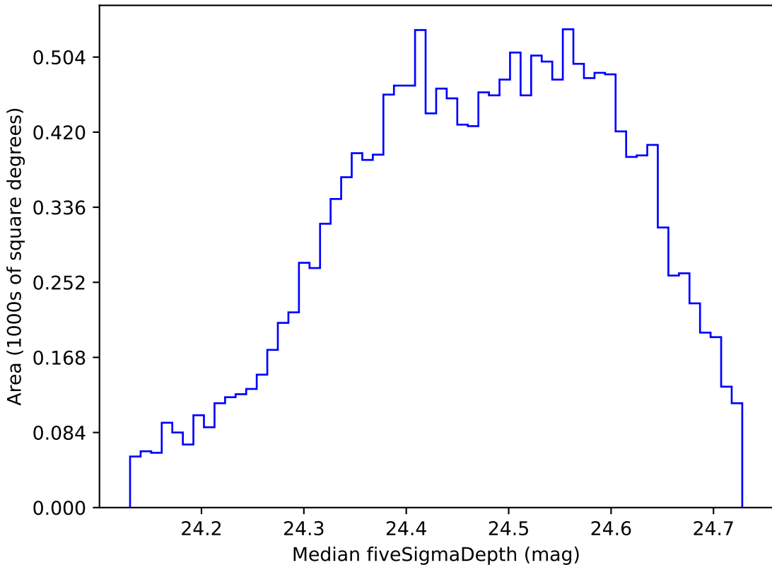
too_ignore_5_1v3.4_10yrs WFD g band: Median fiveSigmaDepth
